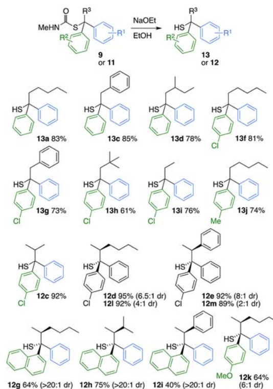
Scheme 4. Tertiary Thiols from Tertiary Thiocarbamates
