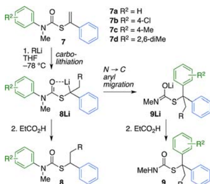
Scheme 2. Carbolithiation–Rearrangement of Thiocarbamates 7
